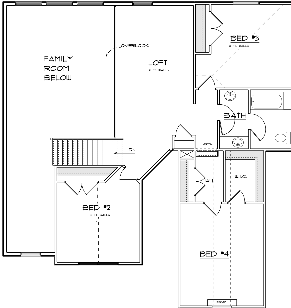
UPPER LEVEL PLAN (1130 SQFT.)
