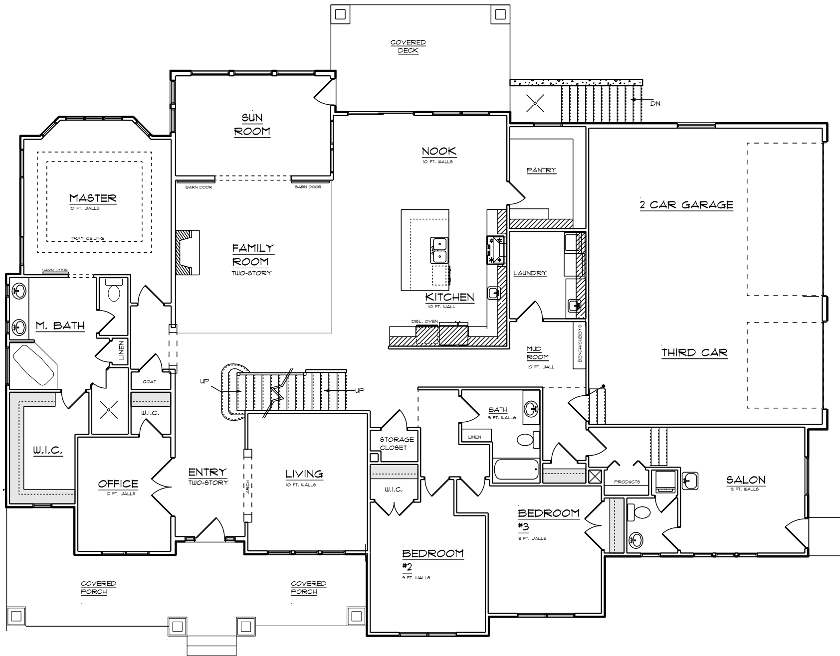
MAIN FLOOR PLAN (3107 SQFT.)
