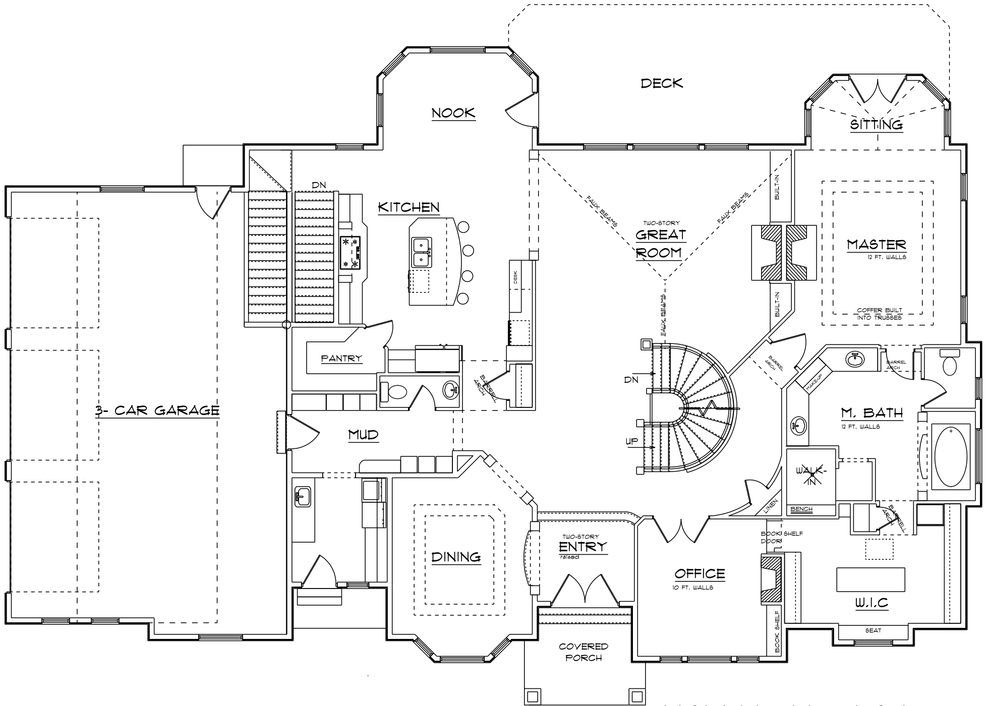
MAIN LEVEL PLAN
