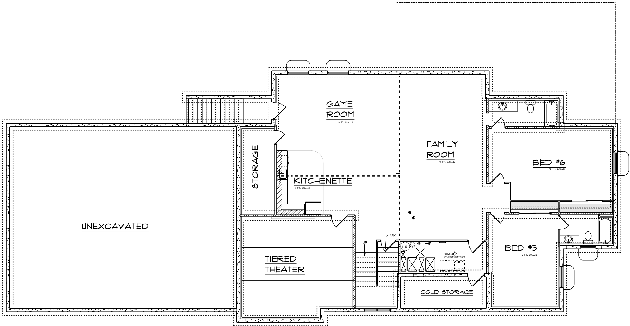
FOUNDATION FLOOR PLAN
