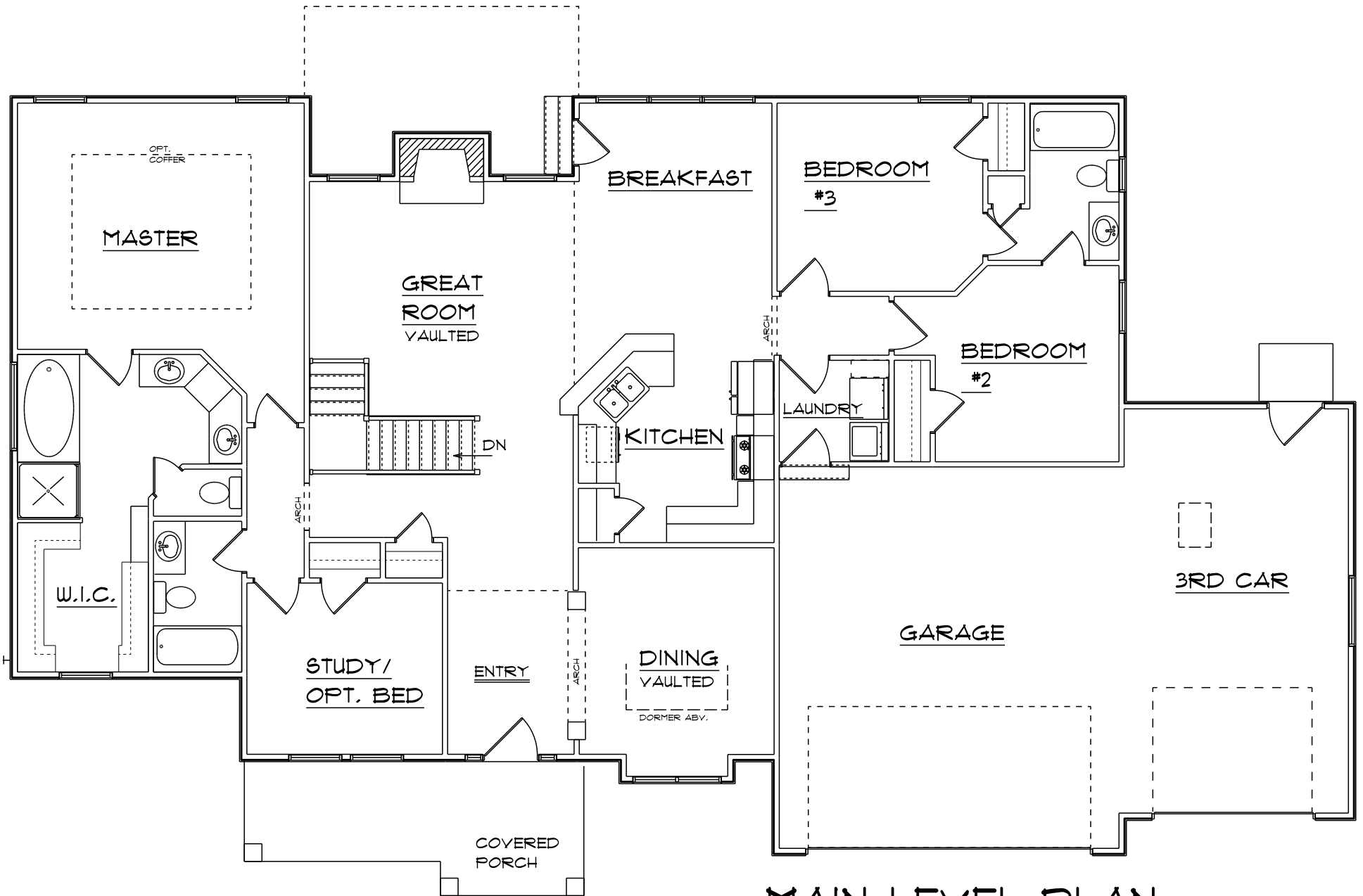
MAIN LEVEL PLAN
