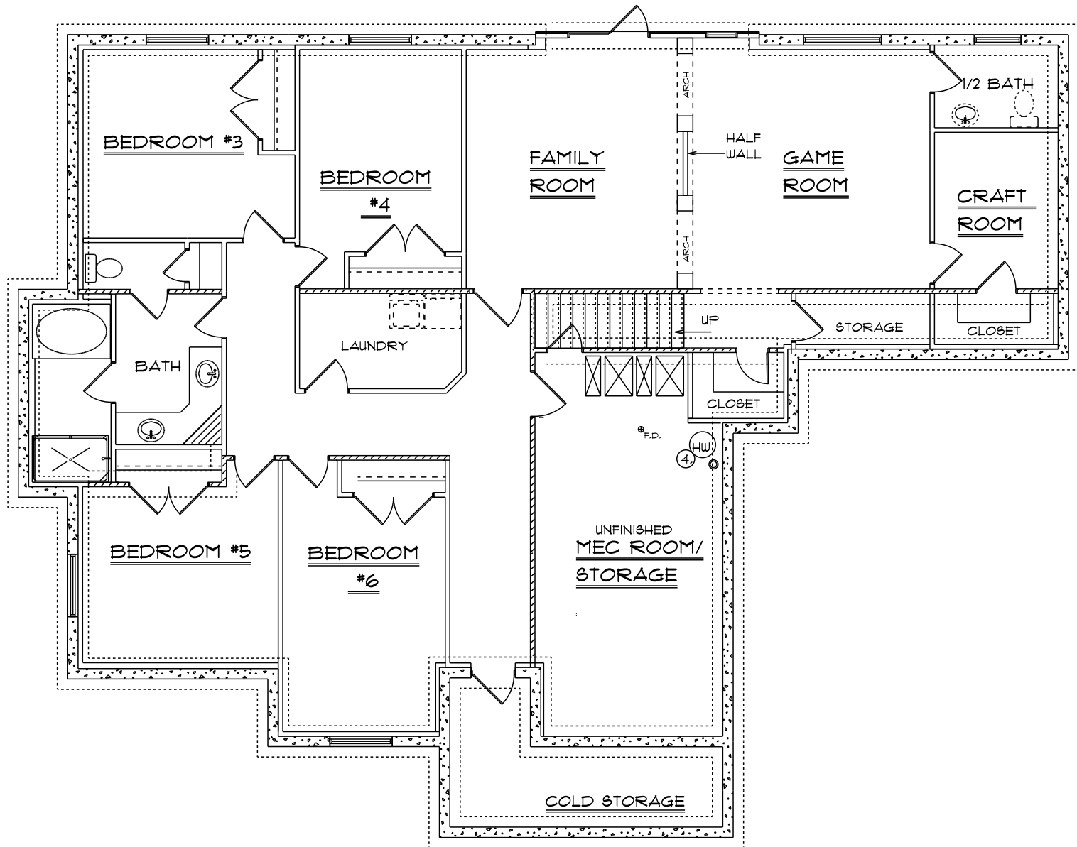
FOUNDATION PLAN
