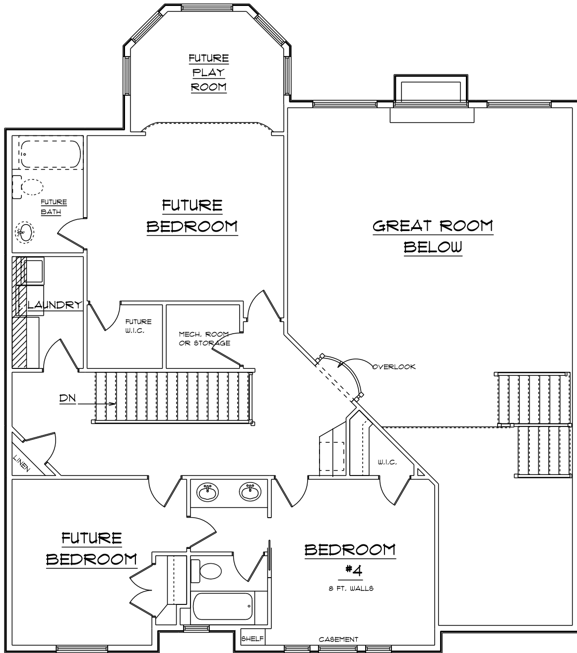
UPPER LEVEL PLAN
