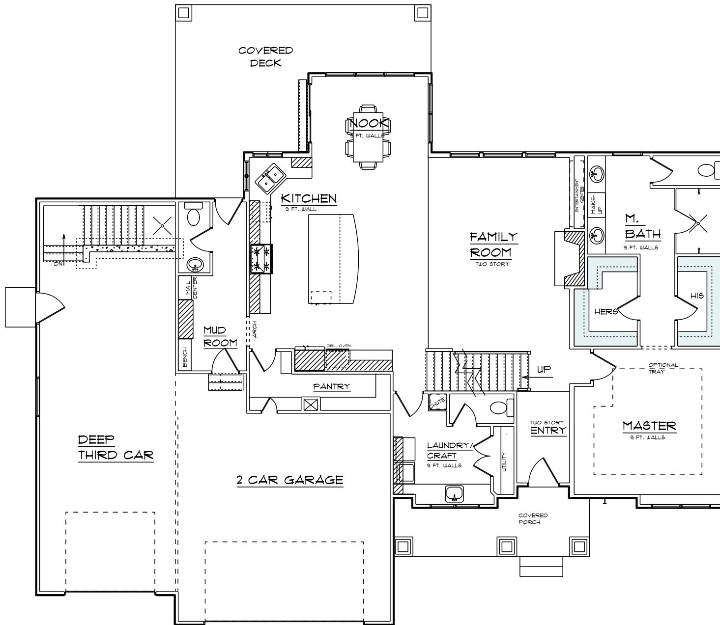
MAIN FLOOR PLAN (1176 SQFT.)
