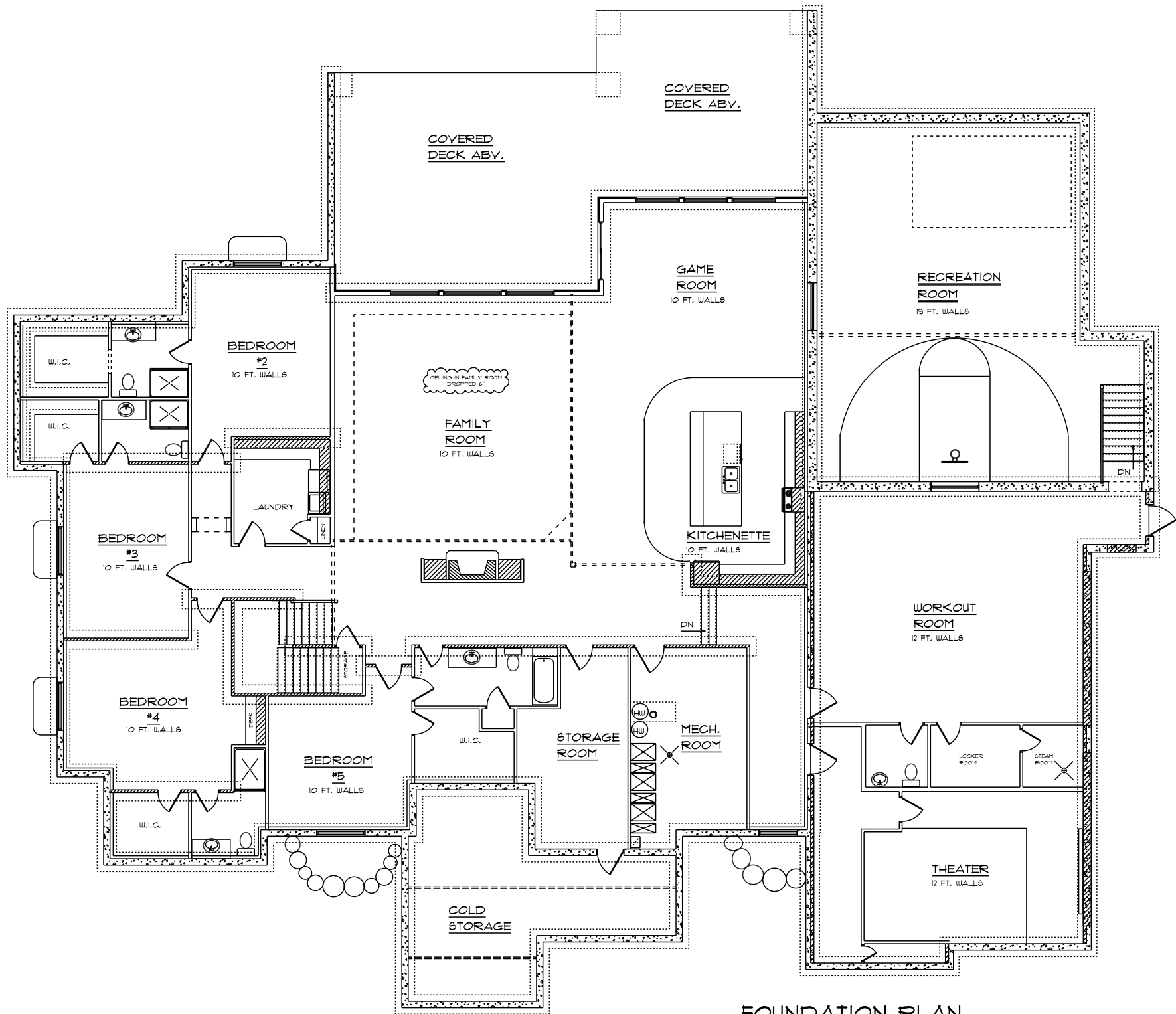
FOUNDATION PLAN
