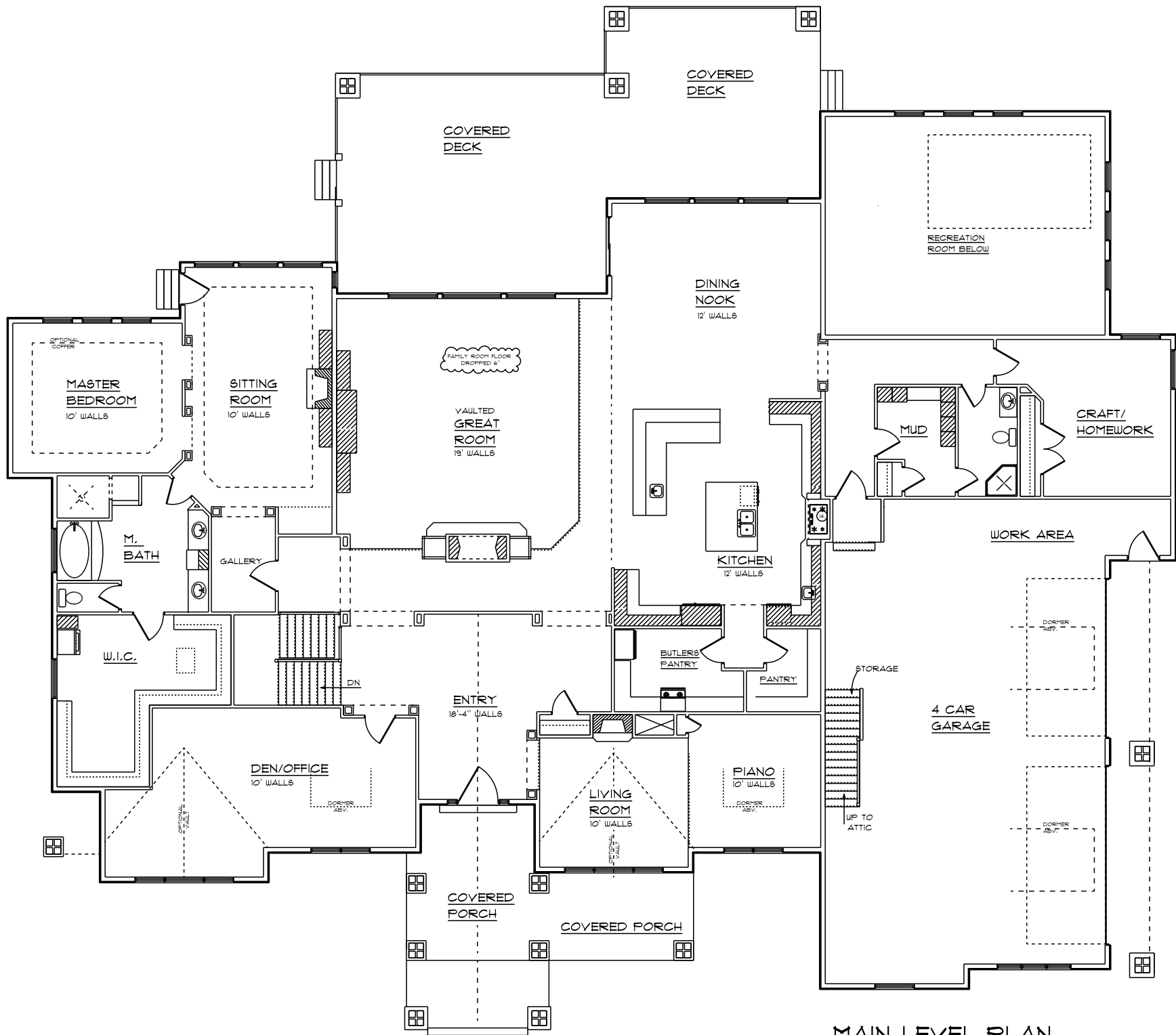
MAIN LEVEL PLAN
