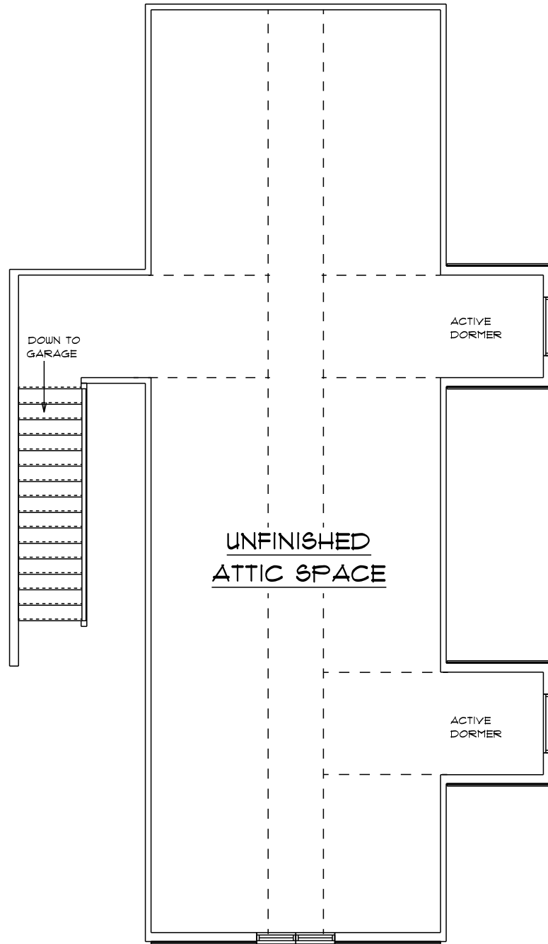
GARAGE ATTIC PLAN
