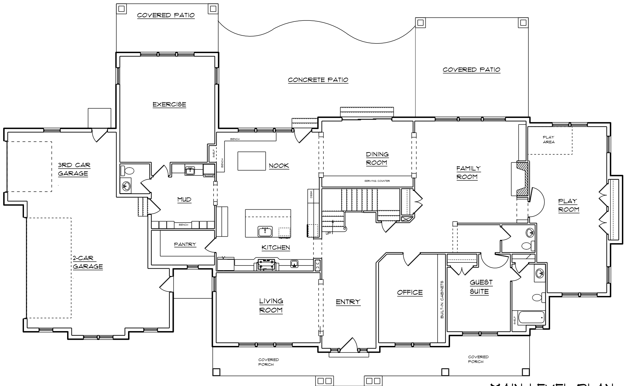
MAIN LEVEL PLAN
